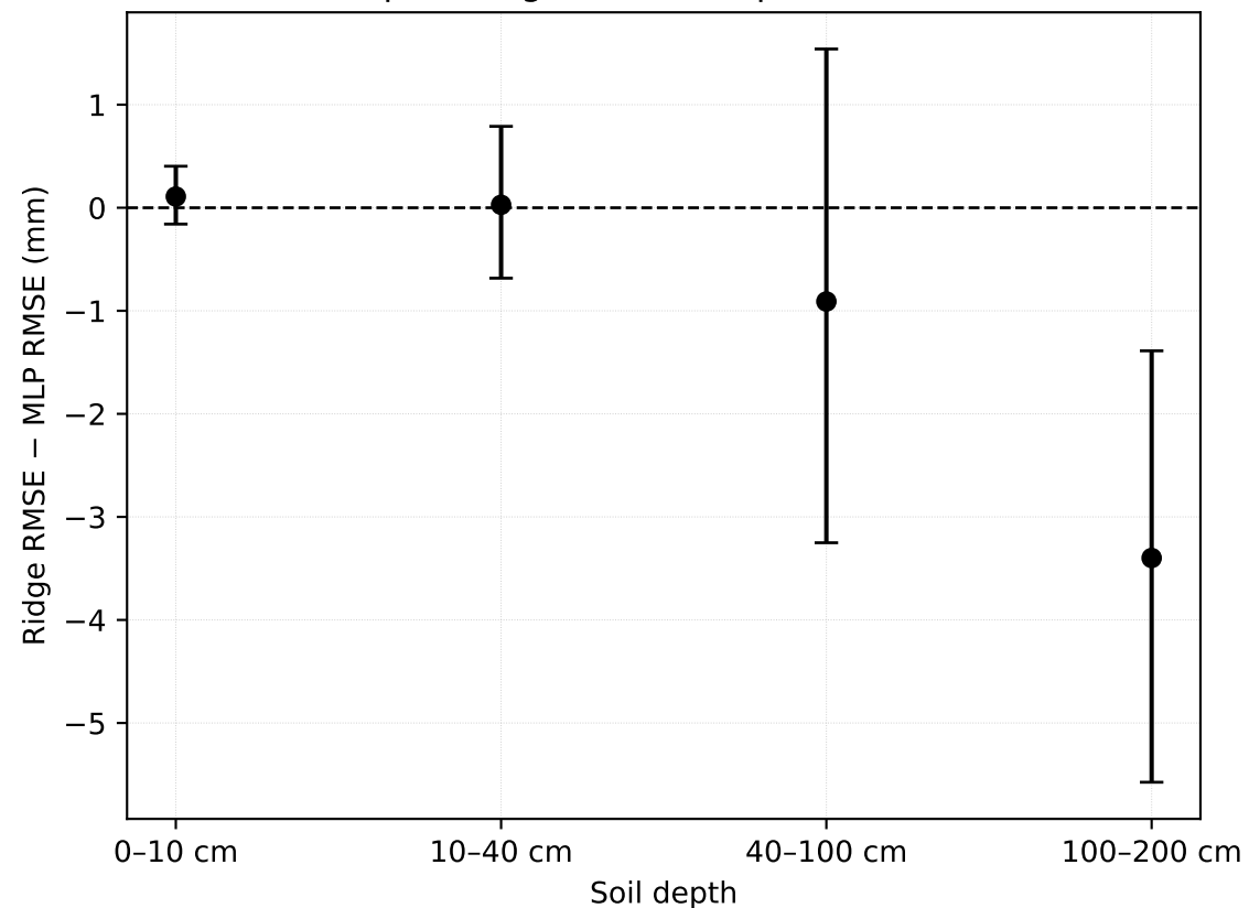
Complete-region bootstrap, 95% interval
