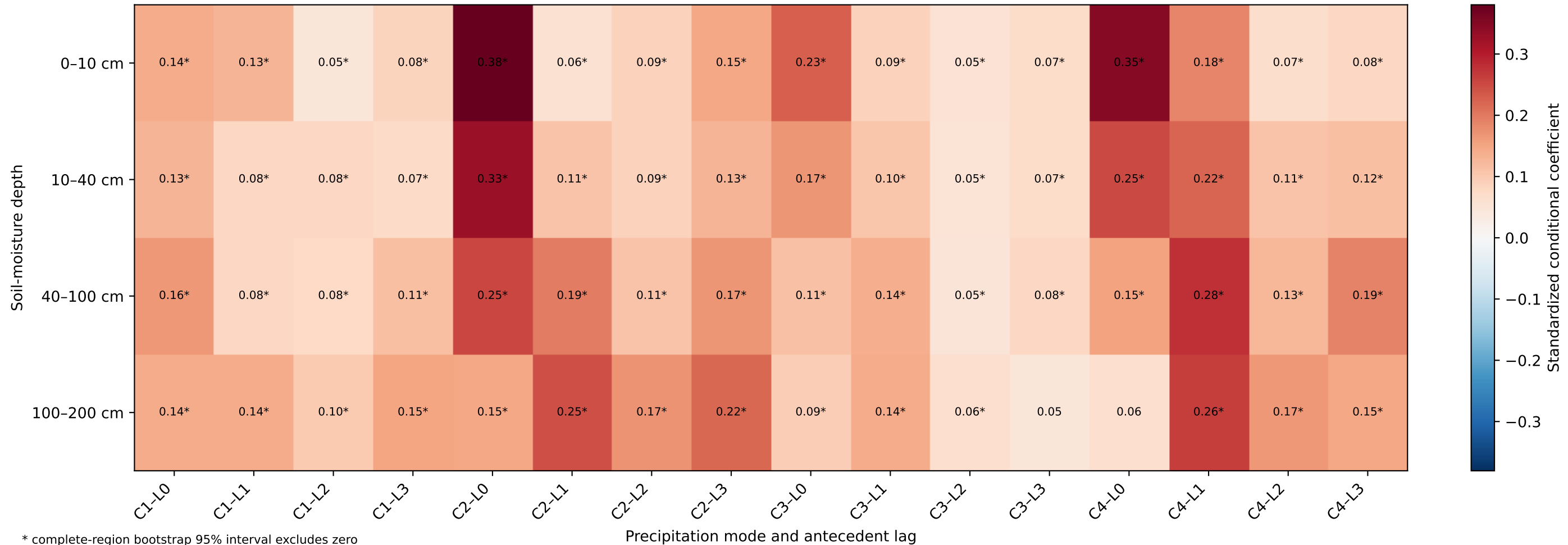
Standardized Ridge attribution across rainfall modes, lags and soil depths
