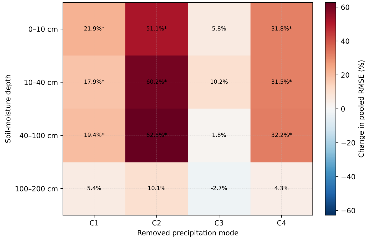
RMSE increase after removing a mode
