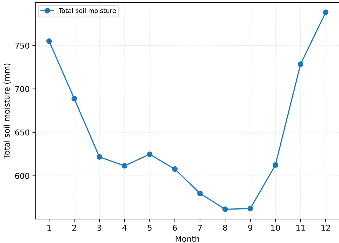
National climatological soil storage
