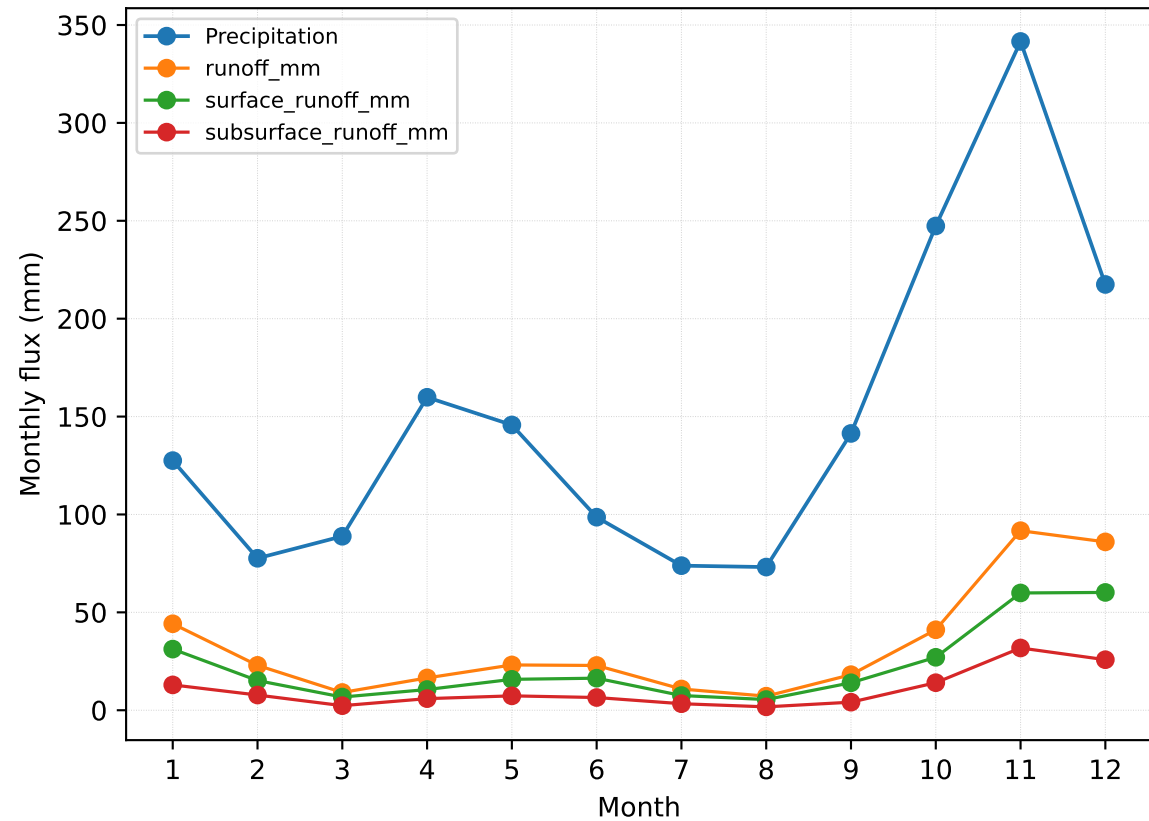
National climatological precipitation and runoff
