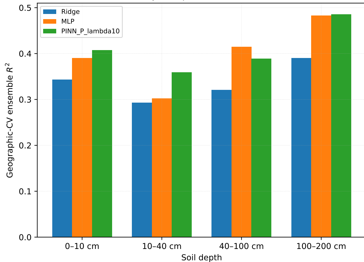
Layer explained variance
