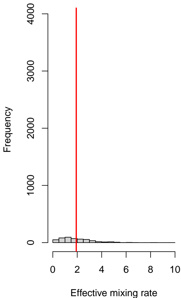
Infectious
