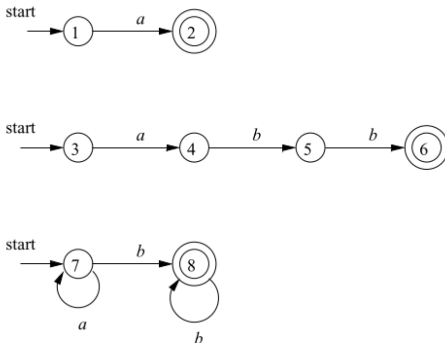
Figure 1: DFAs corresponding to a , abb and a^*b^+
