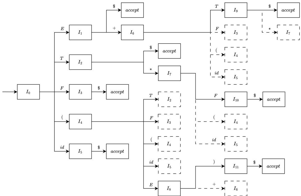
Figure 2: LR(0) automata
