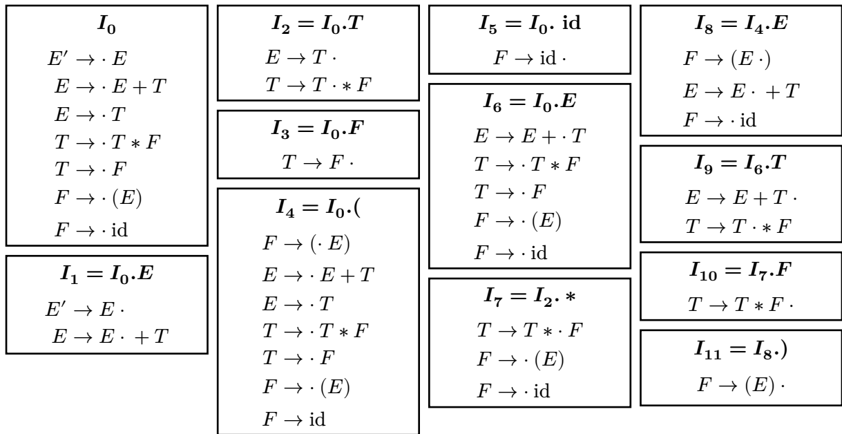
Figure 1: Collection of sets of LR(0) items
