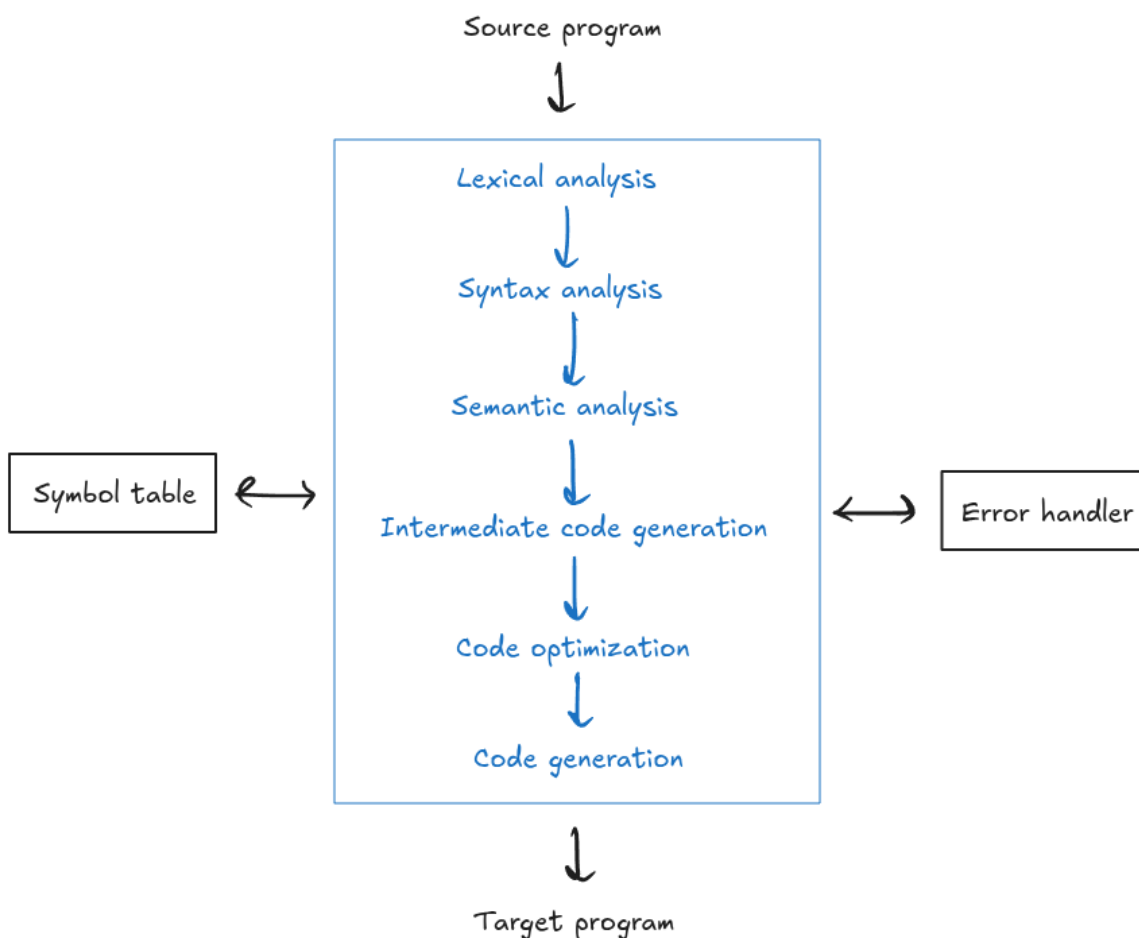
Figure 2: Stages of Compilation
