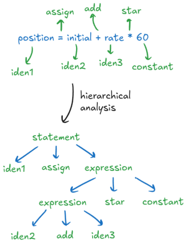
Figure 1: Hierarchical analysis
