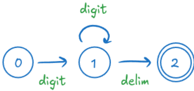
Figure 6: Recognizer for numbers
