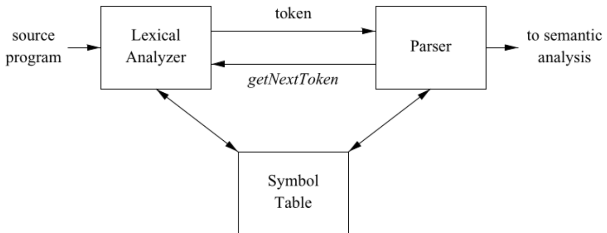
Figure 4: Lexical analyzer
