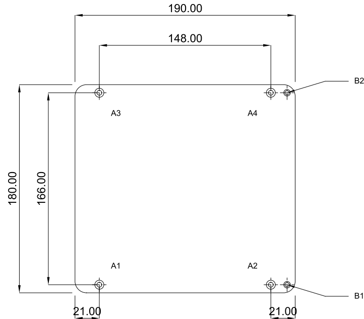
WALL MOUNTING HOLES COVER OPEN / FRONT VIEW
