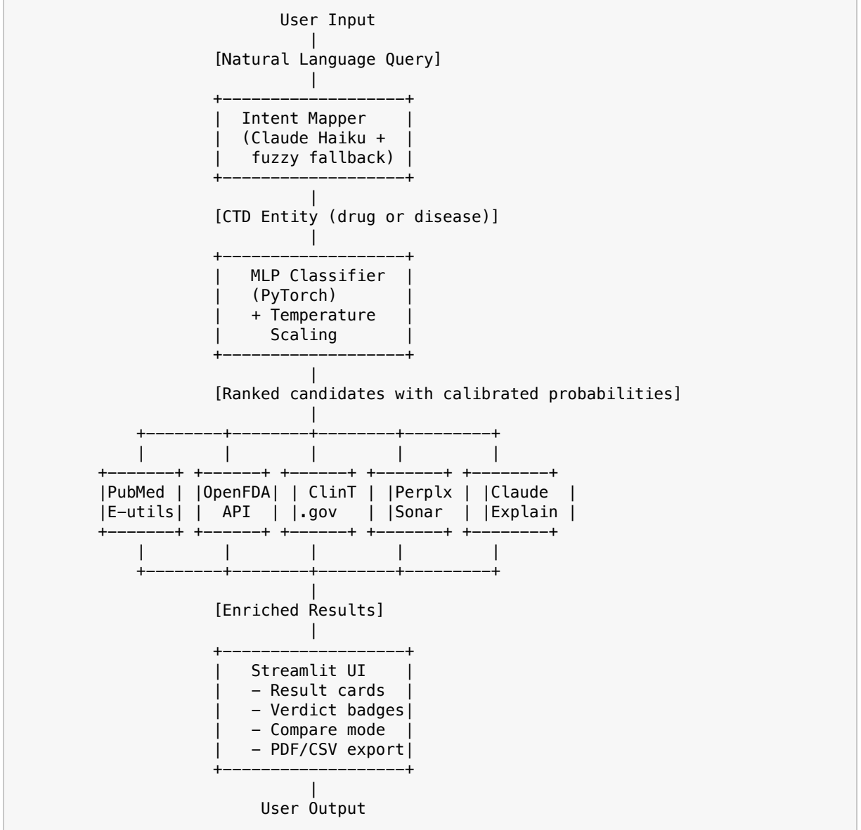
Fig. 1. End-to-end system architecture, showing the flow from natural-language query through intent mapping, MLP scoring, parallel enrichment, and Streamlit rendering.
