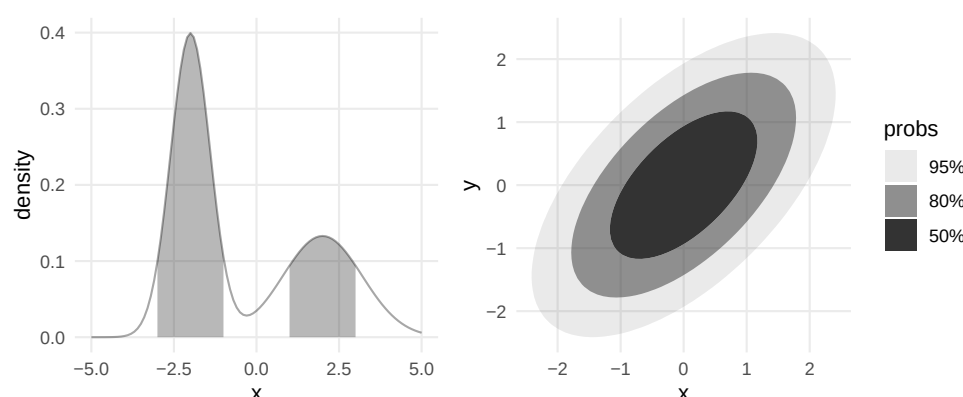
Figure 5: Approximate highest density regions. Left: a disconnected 80% grid-based HDR for a bimodal univariate density. Right: bivariate normal HDRs delegated to ggdensity .
