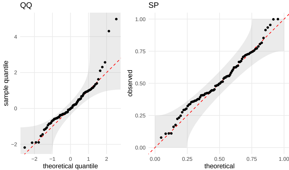
Figure 10: QQ and stabilized probability plots for one sample against a fully specified standard normal null. Fitted-null diagnostics use the same visual band but require separate calibration for formal testing.
