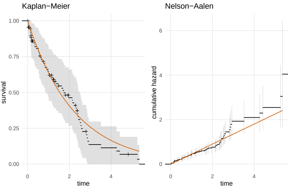
Figure 11: Censored-data summaries from the same simulated sample. The smooth orange curves show the generating \text{Exp}(0.45) survival and cumulative-hazard targets. Left: Kaplan–Meier survival with censor marks and a simultaneous Greenwood/Nair band. Right: Nelson–Aalen cumulative hazard with pointwise normal intervals.
