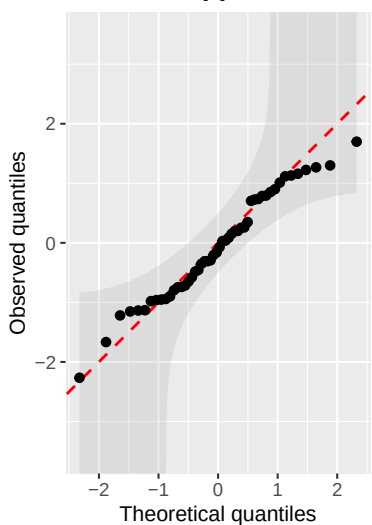
Exponential data: QQ
