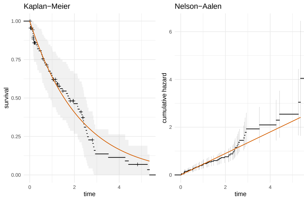
Figure 12: Censored-data summaries from the same simulated sample. Left: Kaplan–Meier survival with censor marks and a simultaneous Greenwood/Nair band. Right: Nelson–Aalen cumulative hazard with pointwise normal intervals.
