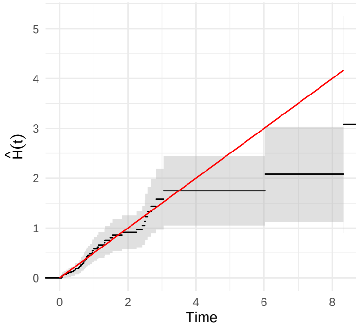
NA vs. Exp(0.5) theory
