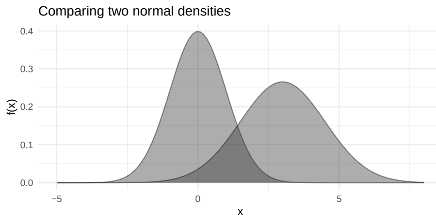
Figure 29: Two normal densities with different means and spreads overlaid in a single plot, demonstrating composability with the ggplot2 grammar of graphics.
