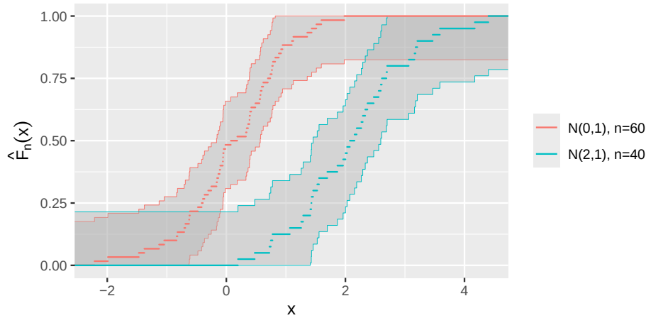
Figure 22: Empirical CDFs for two groups from populations \mathcal{N}(0, 1) and \mathcal{N}(2, 1) , with simultaneous 95% DKW confidence bands. The bands are narrower for larger samples.
