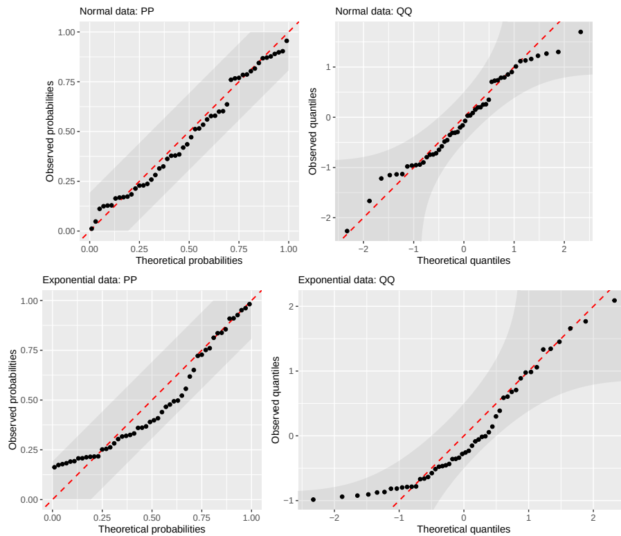
Figure 23: PP and QQ diagnostics for samples compared with a fully specified \mathcal{N}(0, 1) null. The normal sample (top row) follows the identity line and remains within the DKW bands, whereas the shifted exponential sample (bottom row) shows the curvature and tail departures expected from skewness.
