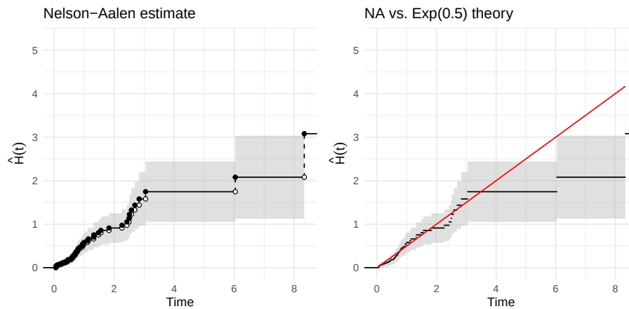
Figure 27: Nelson–Aalen cumulative hazard estimates. The same censored data as in the KM figure. The left panel shows the Nelson–Aalen estimate with a 95% pointwise normal confidence band; the right panel overlays the theoretical H(x) = 0.5x (red).
