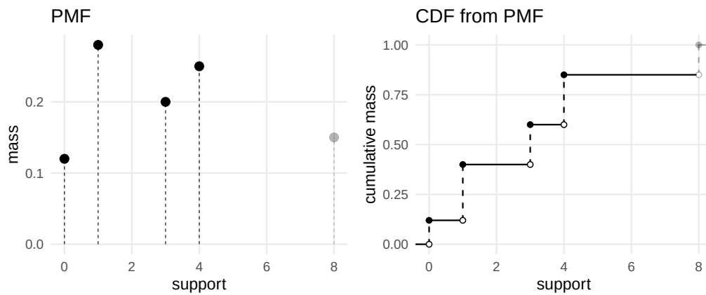
Figure 7: A discrete distribution on a nonconsecutive support. Both layers resolve the same lower cumulative shading request; the discrete CDF is derived from the same PMF by cumulative summation over the declared support.
