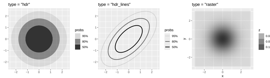
Figure 11: Bivariate normal densities drawn by geom_pdf_2d() : filled 50/80/95% HDRs of the standard bivariate normal (left), HDR boundary lines for a correlated bivariate normal with covariance supplied via args (middle), and a raw density raster with alpha mapped to density (right).
