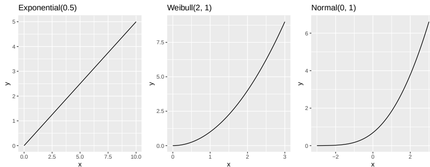
Figure 23: Cumulative hazard functions for three distributions: Exponential(0.5) (left, linear), Weibull(2, 1) (center, convex), and \mathcal{N}(0, 1) (right, eventually superlinear). For the exponential, H(x) = 0.5x confirms the constant hazard rate.
