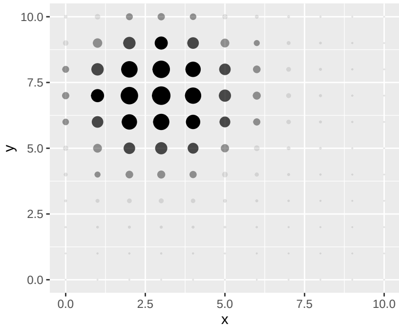
Product binomial, 50/80/95% HDRs
