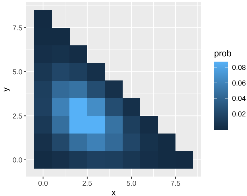
Trinomial on a simplex
