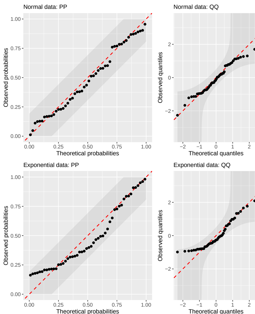
Figure 23: PP and QQ diagnostics for samples compared with a fully specified \mathcal{N}(0, 1) null. The normal sample (top row) follows the identity line and remains within the DKW bands, whereas the shifted exponential sample (bottom row) shows the curvature and tail departures expected from skewness.
