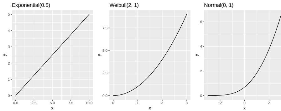
Figure 21: Cumulative hazard functions for three distributions: Exponential(0.5) (left, linear), Weibull(2, 1) (center, convex), and \mathcal{N}(0, 1) (right, eventually superlinear). For the exponential, H(x) = 0.5x confirms the constant hazard rate.
