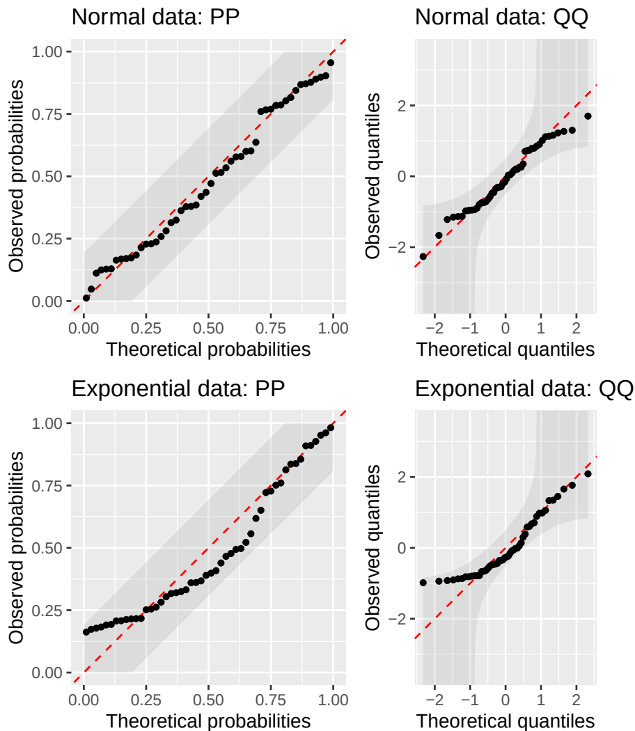
Figure 23: PP and QQ diagnostics for samples compared with a fully specified \mathcal{N}(0,1) null. The normal sample (top row) follows the identity line and remains within the DKW bands, whereas the shifted exponential sample (bottom row) shows the curvature and tail departures expected from skewness.
