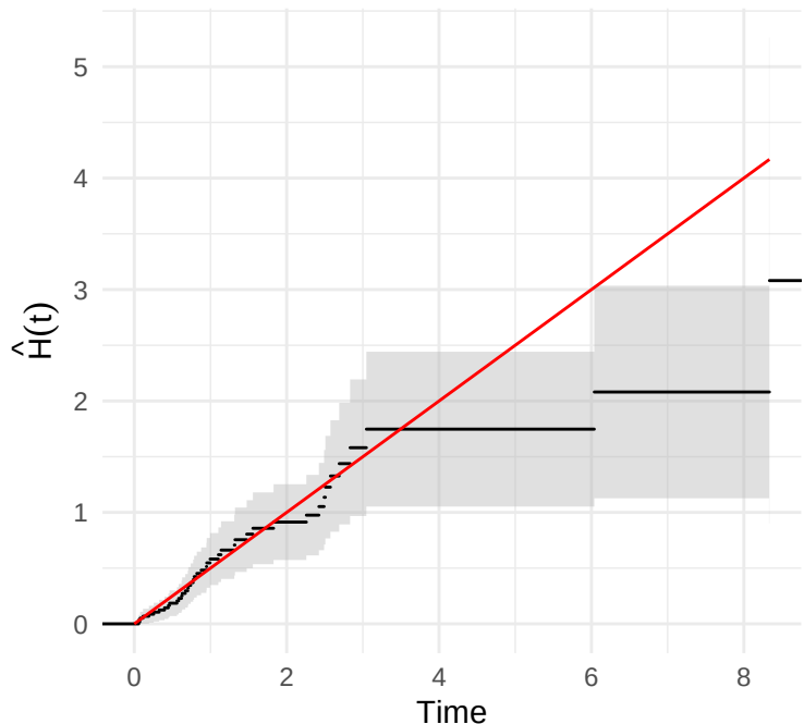
NA vs. Exp(0.5) theory
