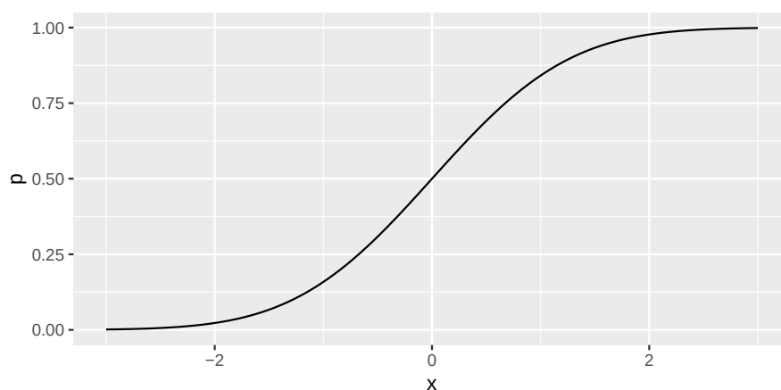
Figure 16: The standard normal CDF.
