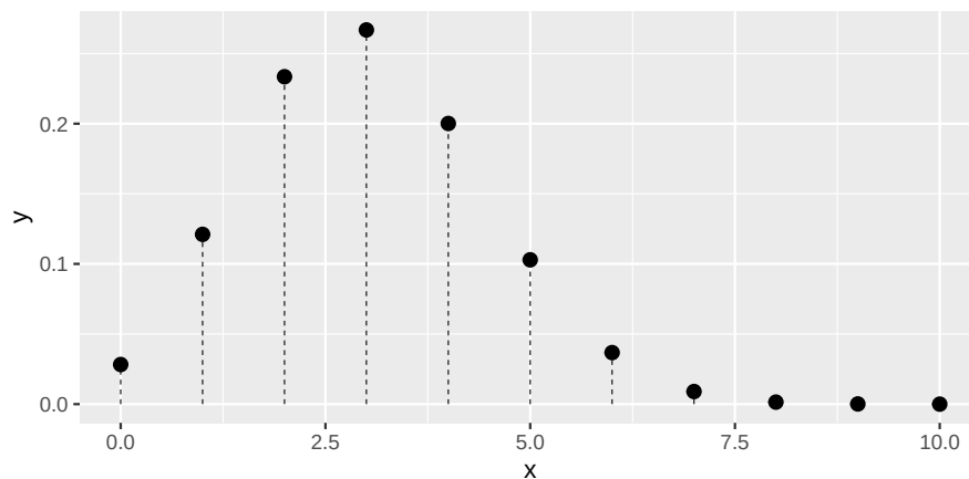
Figure 12: The PMF of a \text{Binomial}(10, 0.3) distribution, rendered as a lollipop chart.
