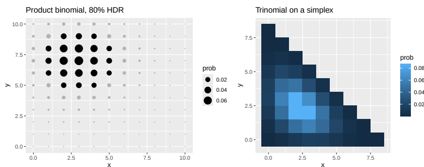
Figure 15: Bivariate PMFs rendered by geom_pmf_2d() : the 80% highest density region of a product \text{Binomial}(10, 0.3) \times \text{Binomial}(10, 0.7) distribution in the default balloon rendering, with lattice points outside the HDR greyed (left), and a trinomial distribution with n = 8 evaluated over a bounding lattice in the tile rendering, showing only its simplex support (right).
