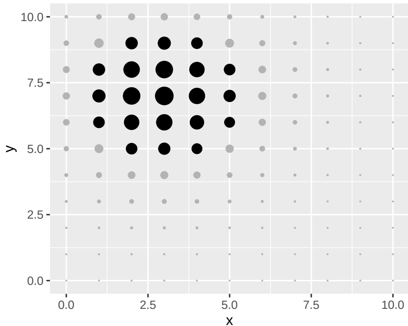
Product binomial, 80% HDR
