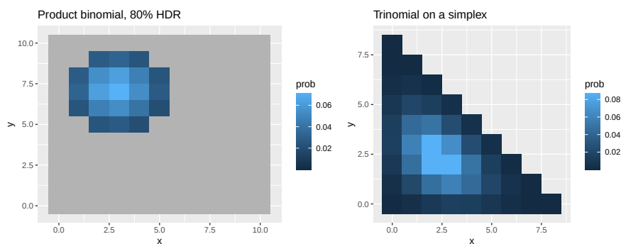
Figure 15: Bivariate PMFs rendered by geom_pmf_2d() : the 80% highest density region of a product Binomial(10,0.3) \times Binomial(10,0.7) distribution, with lattice points outside the HDR greyed (left), and a trinomial distribution with n = 8 evaluated over a bounding lattice, rendering only its simplex support (right).
