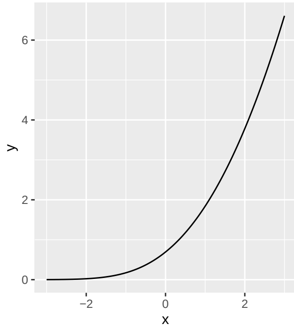
Normal(0, 1)
