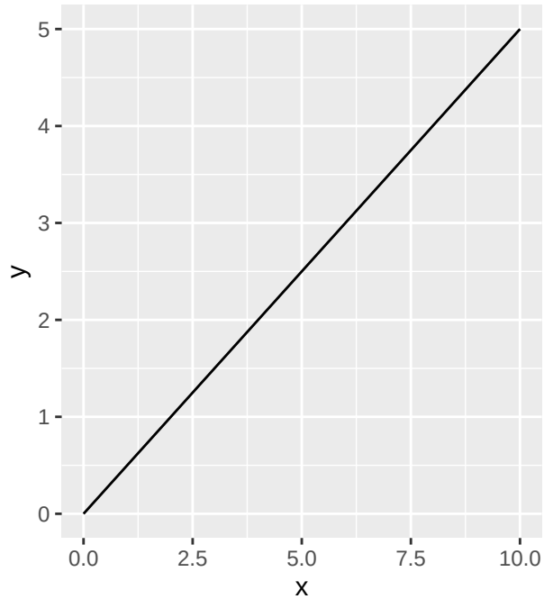
Exponential(0.5)
