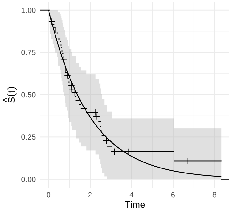
KM vs. Exp(0.5) theory
