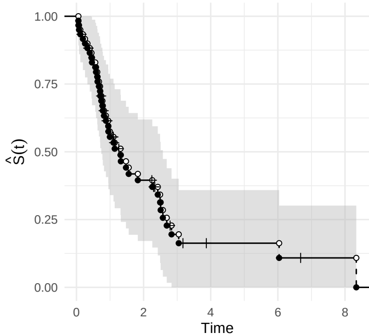
Kaplan–Meier estimate
