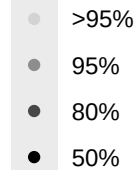
probs
