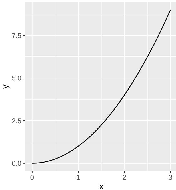
Weibull(2, 1)
