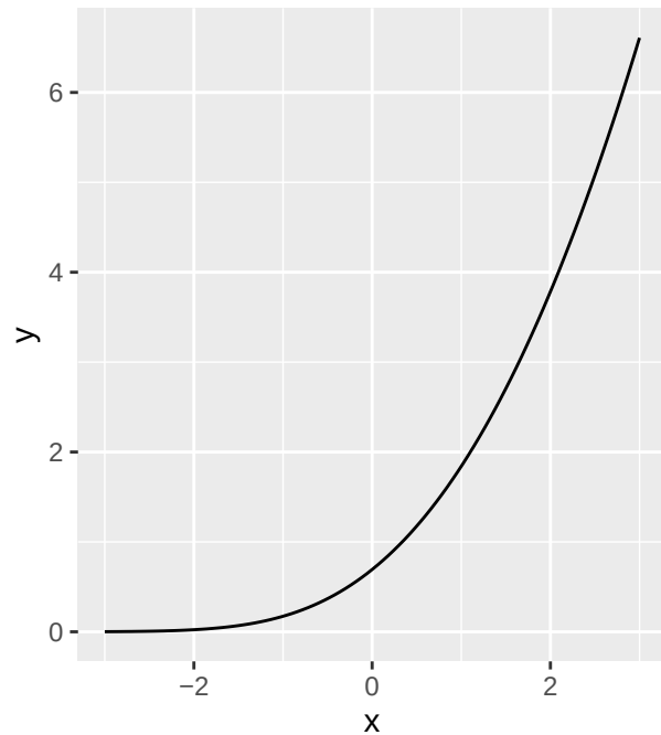
Normal(0, 1)
