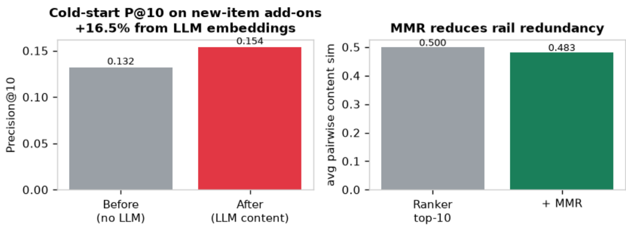
Fig 4. LLM content embeddings lift cold-start new-item Precision@10 by +16.5%; MMR cuts rail redundancy.
