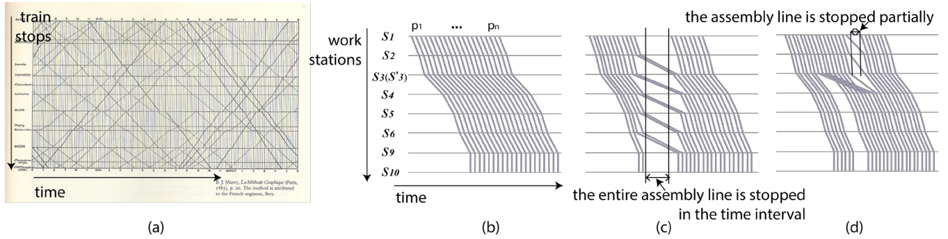
Fig. 3. Marey's graph [29] and the relevant visual patterns when applied to the manufacturing process data. It uses the path (s_1, s_2, s_3(s'_3), s_5, s_6, s_9, s_{10}) in the DAG in Fig. 2 for illustration. (a) the original Marey's graph shows the bus/train schedules; (b) Marey's graph showing when a product starts being processed on each work station on an assembly line, the visual pattern shows that no abnormal delay has occurred and the assembly line works smoothly; (c) the assembly line is completely stopped during a time interval, which can be caused by faults or prescheduled maintenance; (d) the assembly line is partially stopped to handle unprocessed products.
