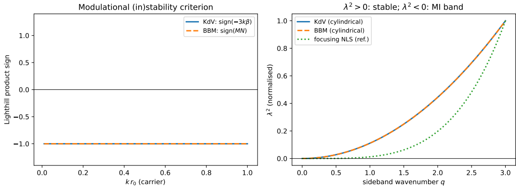
FIGURE 8 Modulational (in)stability of the cylindrical reductions for the physiological parameters of Figure 4 ( \gamma = 0 ). Left: the sign of the Lighthill product ( -3k\beta for KdV, MN for BBM) is negative across the long-wave range, so both envelopes are defocusing. Right: \lambda^2(q) remains positive for the KdV and BBM reductions (empty instability band), in contrast with a focusing reference NLS (dotted), whose \lambda^2 becomes negative. Produced by scripts/mi_growth.py .
