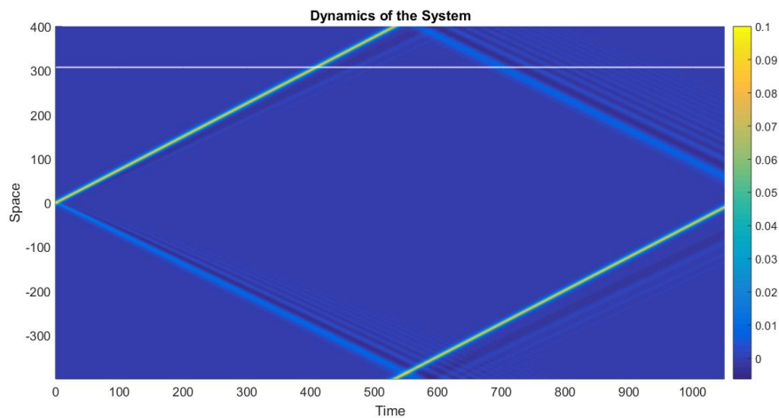
FIGURE 5 Space-time plot of the KdV soliton (120) evolution under the Boussinesq system (115)–(116) dynamics for initial amplitude A = 0.1 from t = 0 to t = 1050 . Parameters are reported in Table 1.
