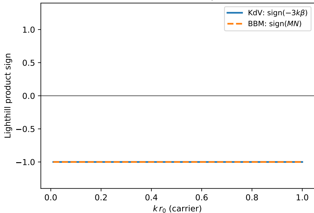
Modulational (in)stability criterion
