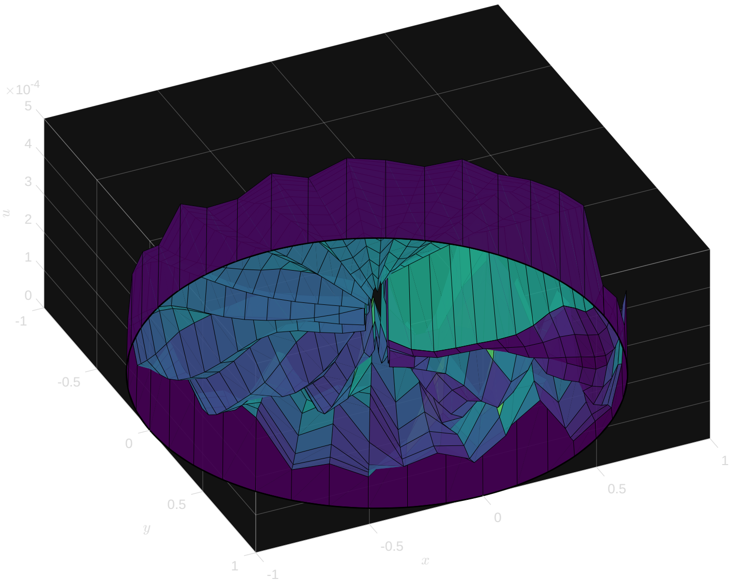
Poisson equation on the disk: off-centre Gaussian load
