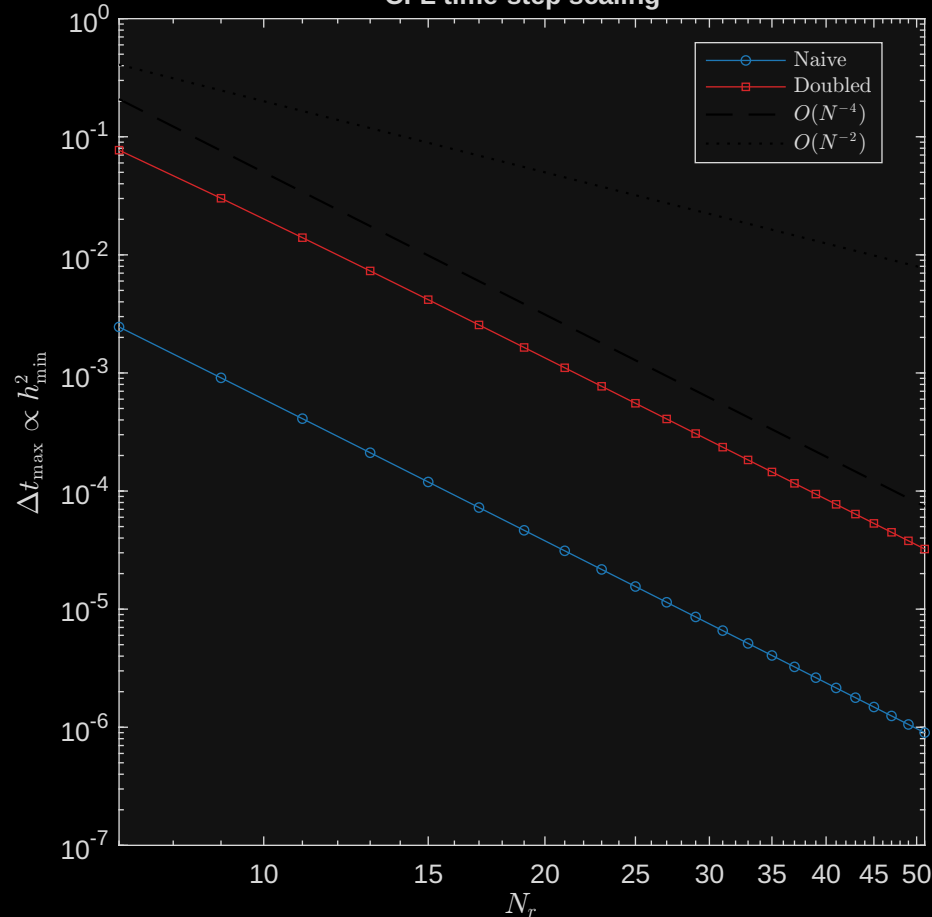
CFL time-step scaling
