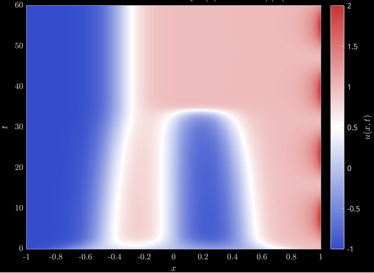
Allen–Cahn: Driven Boundary u(1) = 1 + \sin^2(t/5)
