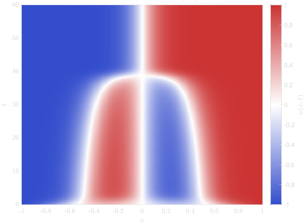
Allen-Cahn: Fixed Boundaries u(\pm 1) = \pm 1
