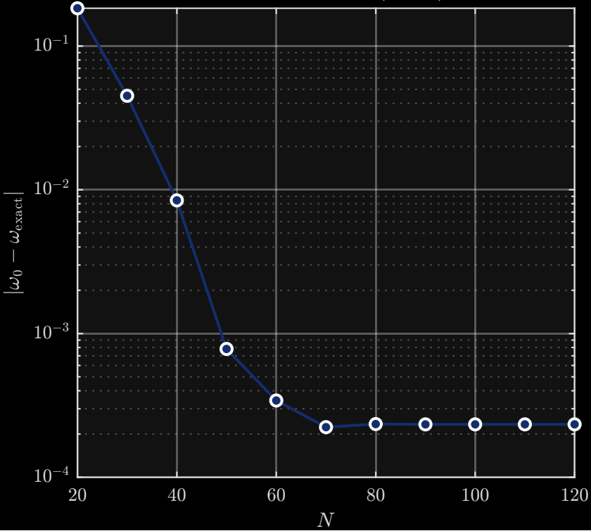
Convergence vs N ( L = 8 )
