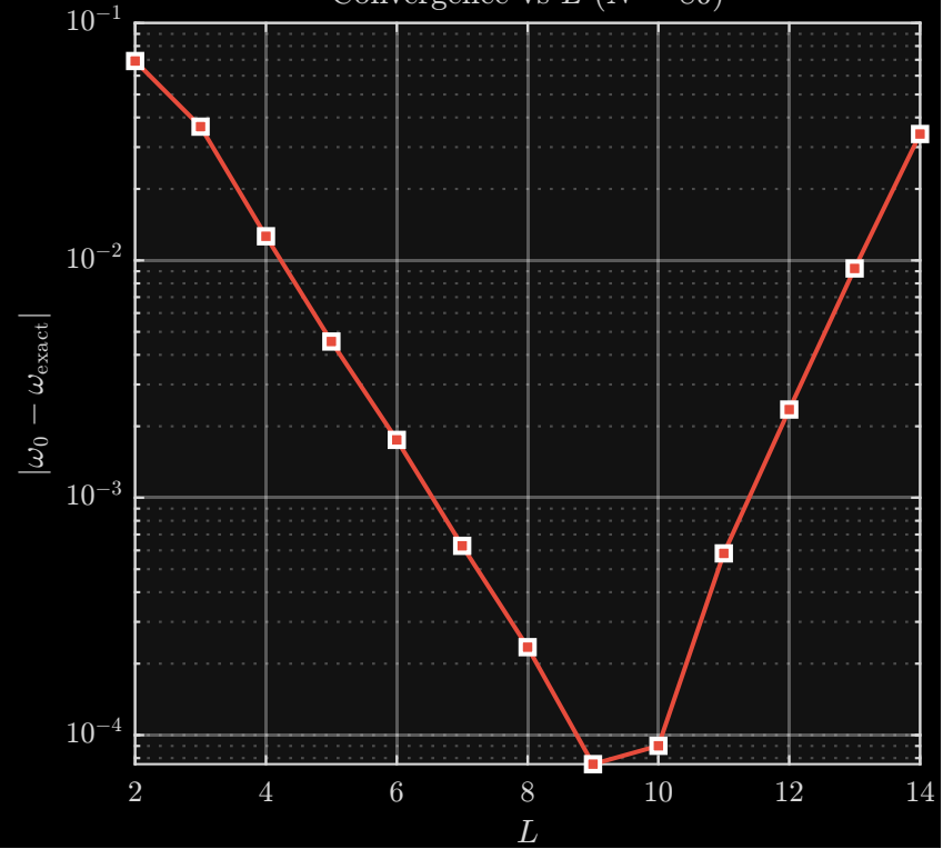
Convergence vs L ( N = 80 )
