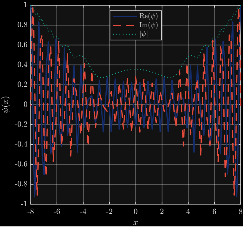
Mode 1: \omega = -9.7068 - 0.2068i
