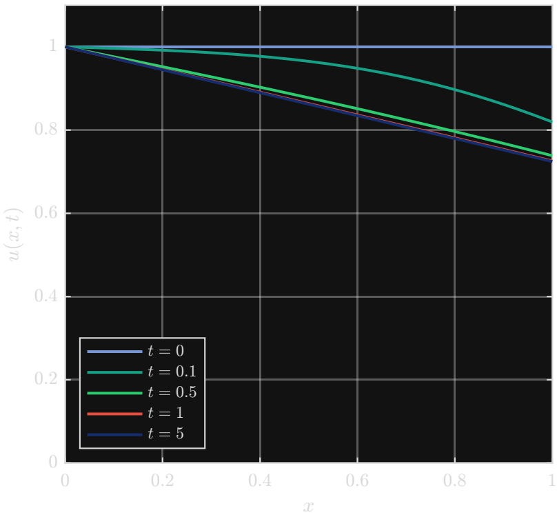
Temperature Profiles ( \sigma = 1 )
