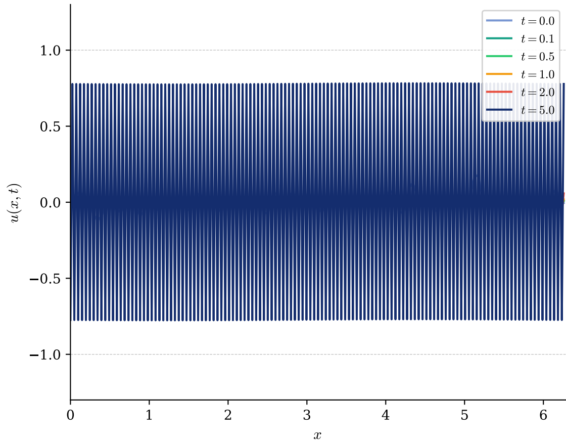
Snapshots at Selected Times
