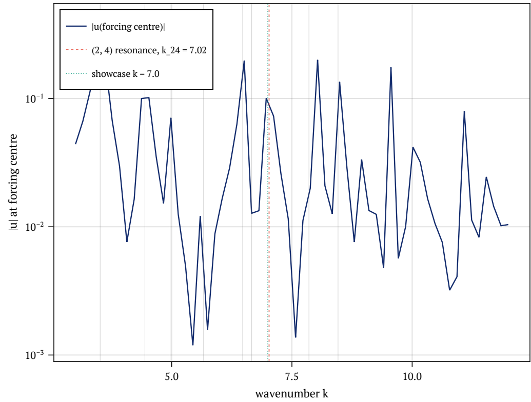
(c) resonance amplification of |u| vs k
