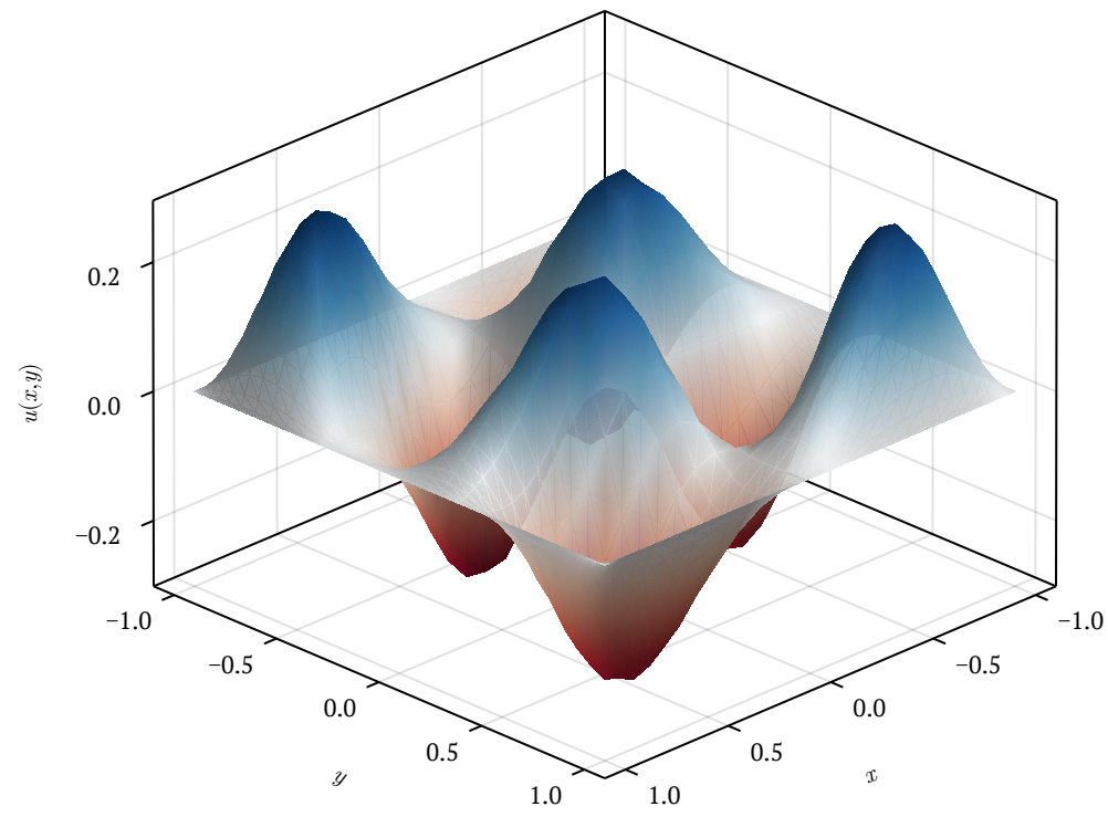
(a) Solution surface (k = 7)
