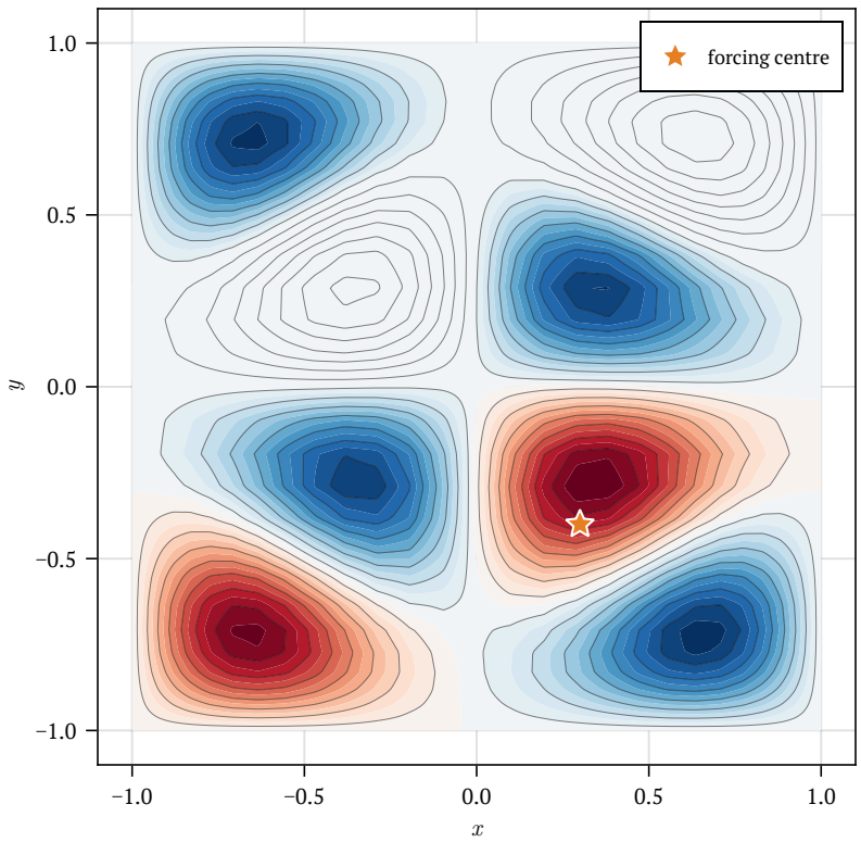
(b) Contour of solution
