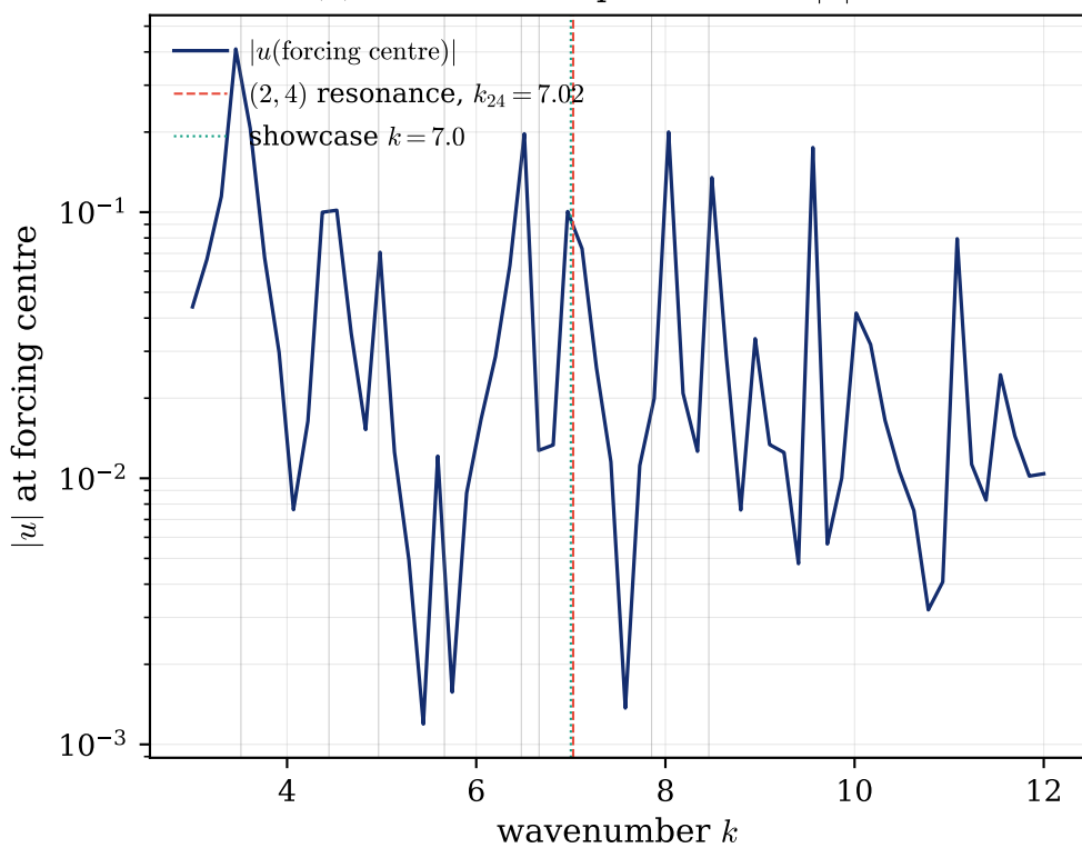
(c) resonance amplification of |u| vs k
