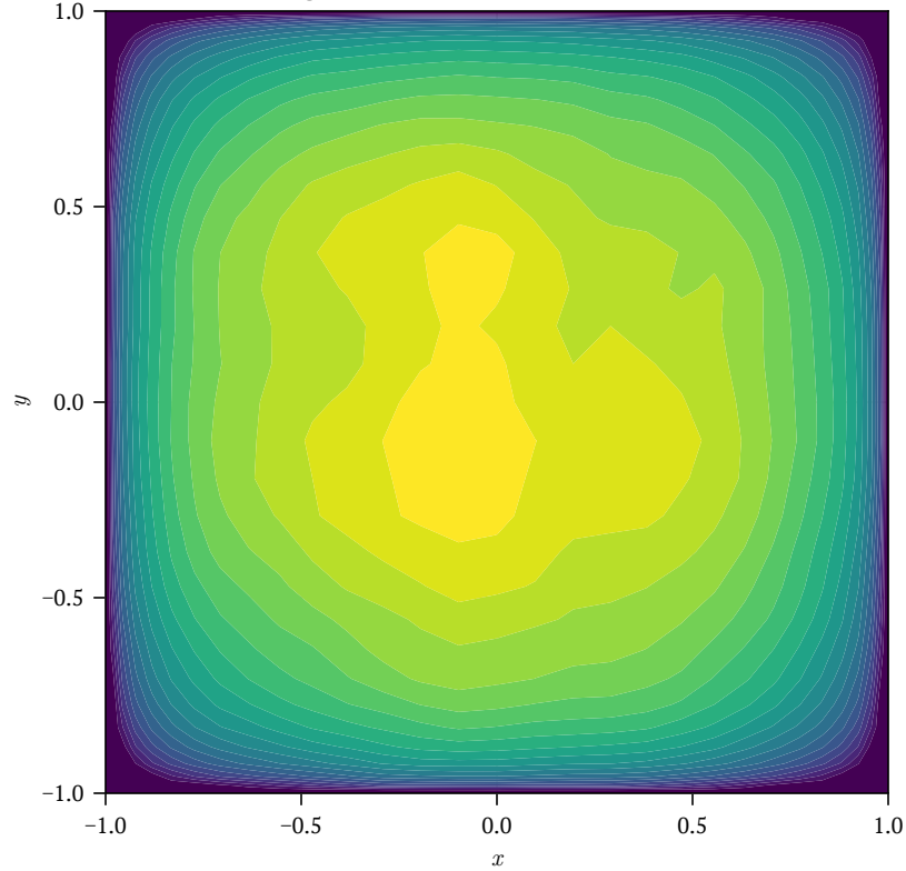
(c) \log_{10} |u_N - u_{\text{exact}}| (max = 1.12\text{e-}14 )
