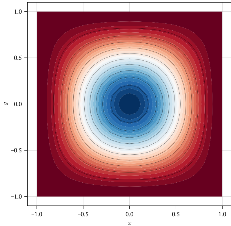
(c) \log_{10} |u_N - u_{\text{exact}}| (max = 1.12\text{e-}14 )
