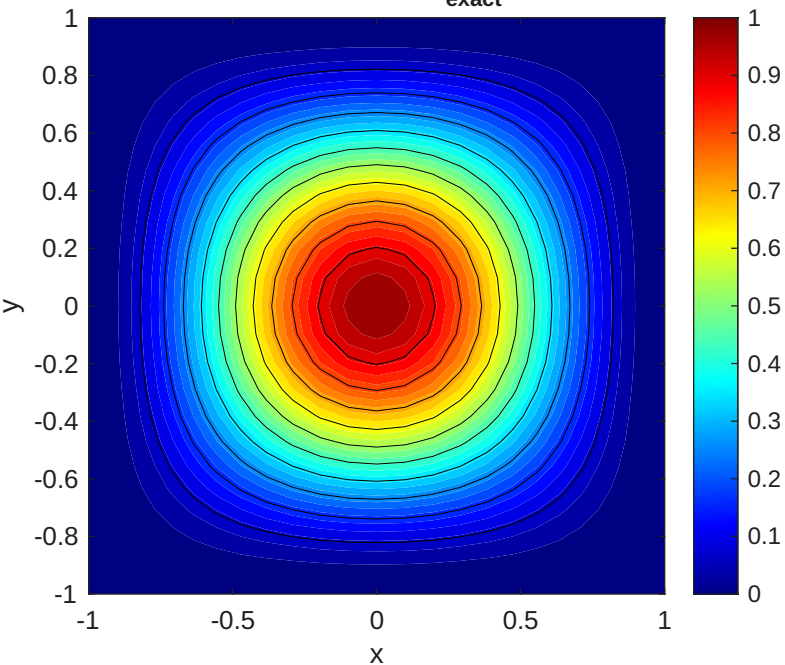
(a) Exact solution u_{\text{exact}}(x, y)
