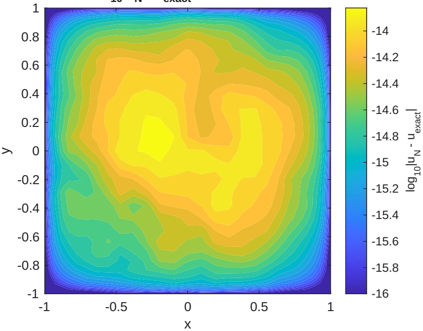
(c) \log_{10}|u_N - u_{\text{exact}}| (max = 1.92\text{e-}14 )
