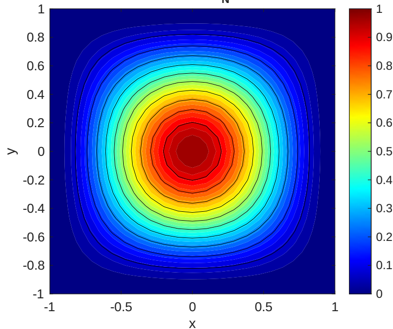
(b) Numerical solution u_N(x, y) at N = 32
