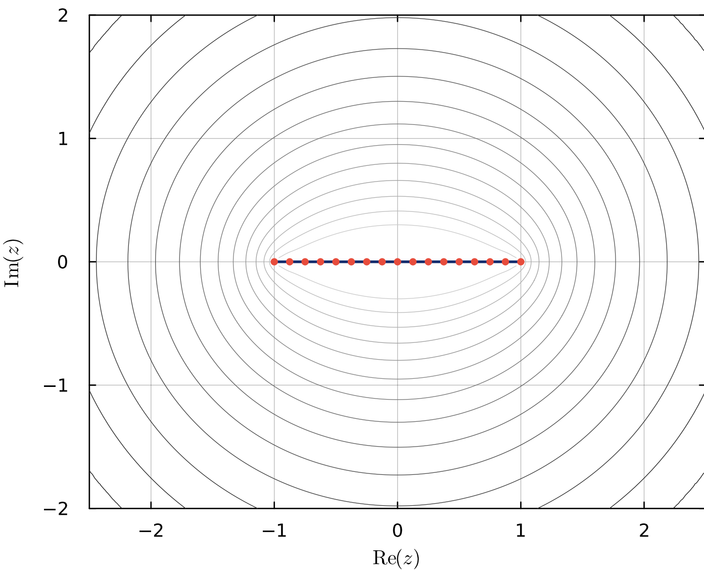
(c) Clenshaw-Curtis
