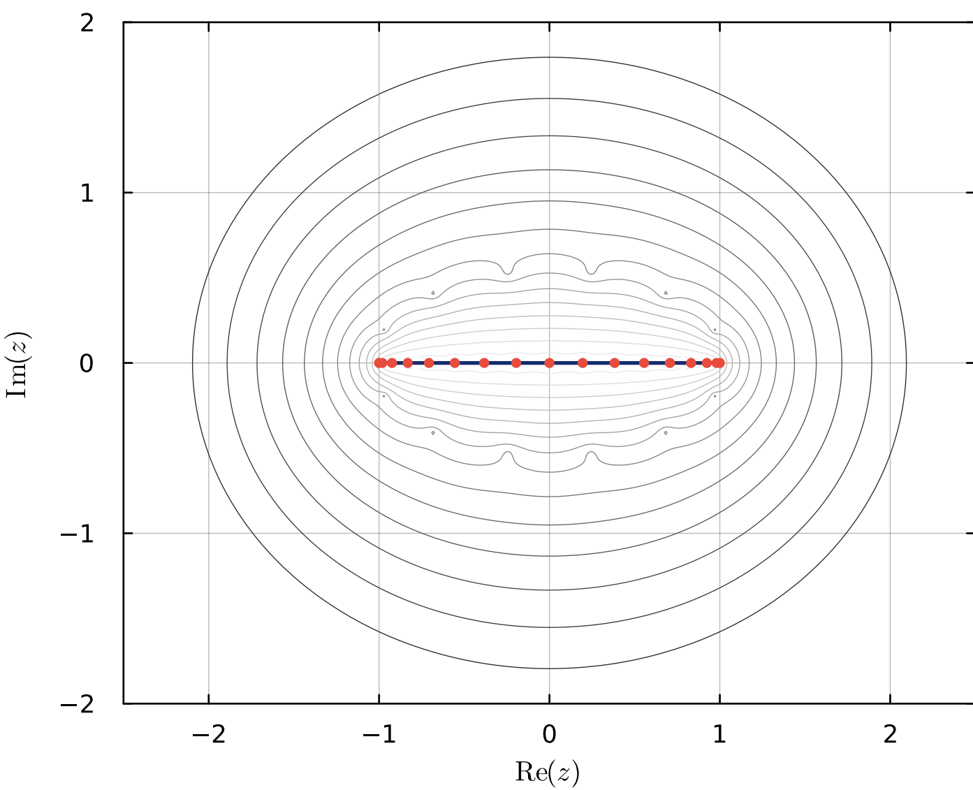
(c) Clenshaw-Curtis
