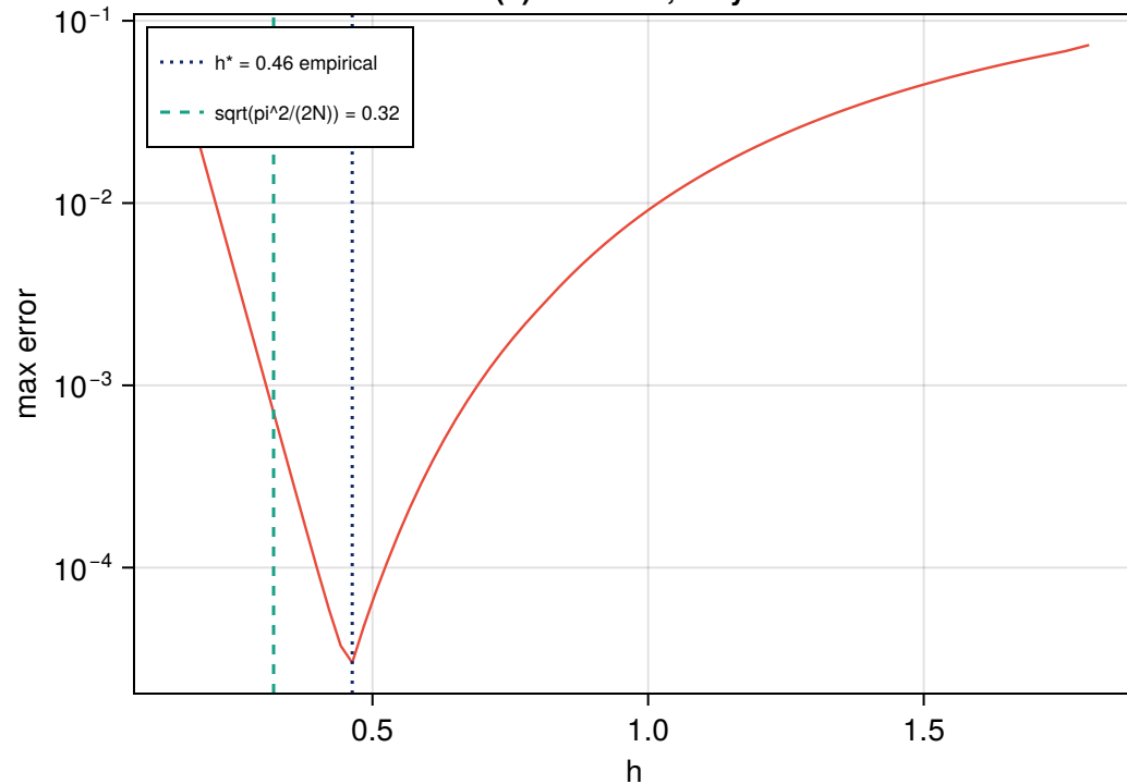
(c) Subgeometric convergence at h = h^*
