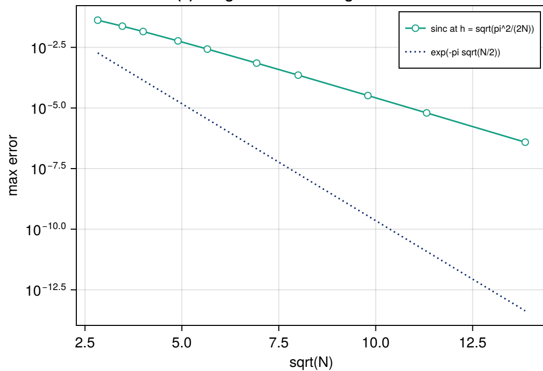
(c) Subgeometric convergence at h = h^*
