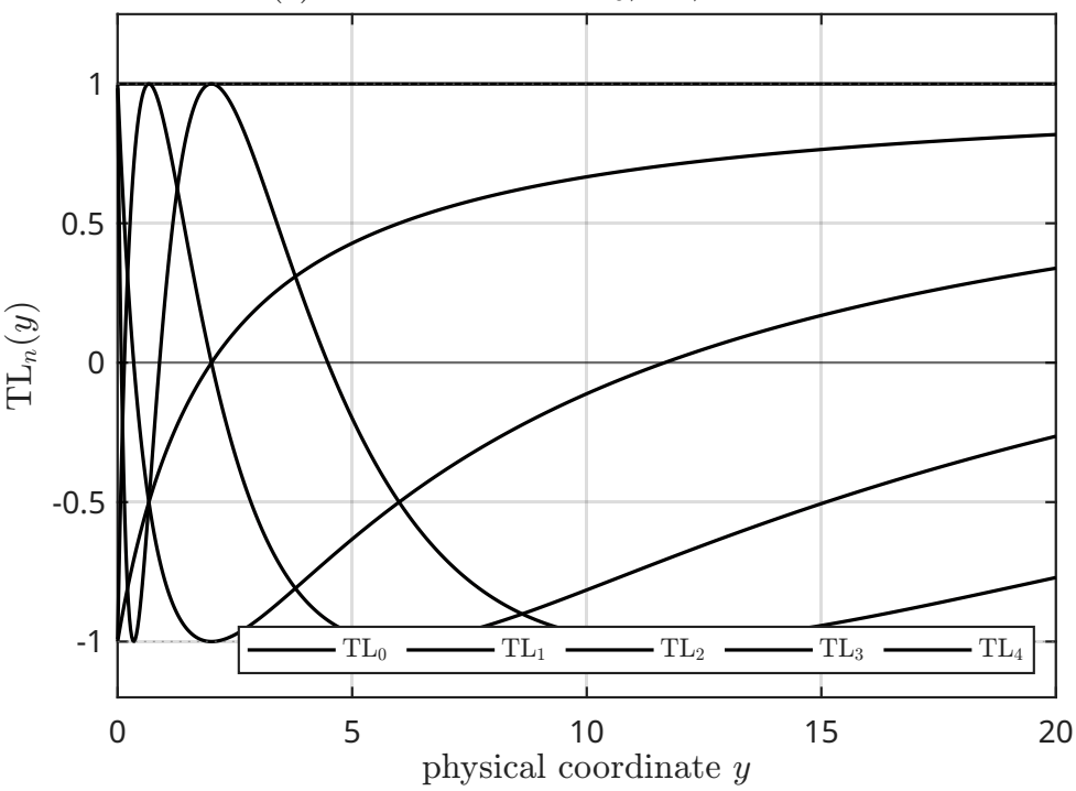
(c) basis functions \text{TL}_0, \dots, \text{TL}_4 at \ell = 2
