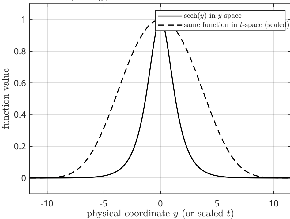
(c) \text{sech}(y) in two coordinate frames at \ell = 1
